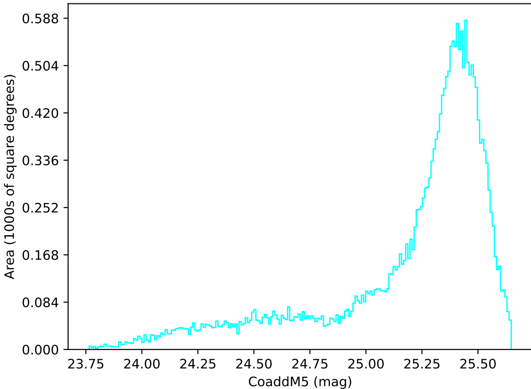
too_elab_r32_d2_griz_v3.4_10yrs All sky u band: CoaddM5
