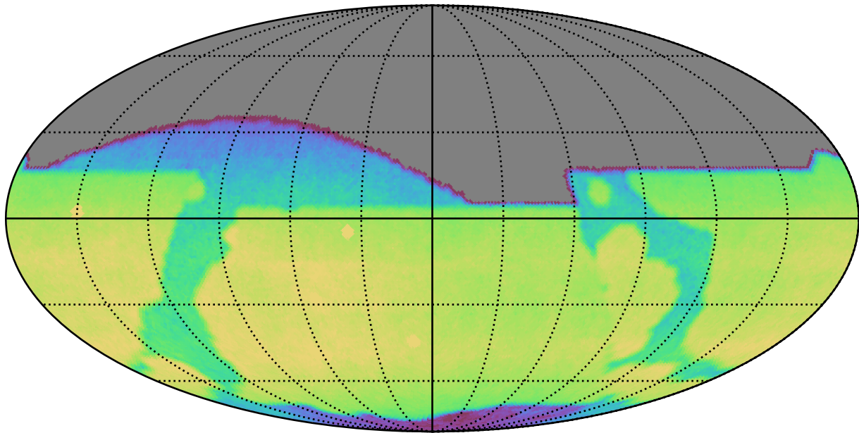
too_elab_r32_d2_griz_v3.4_10yrs All sky r band: CoaddM5
