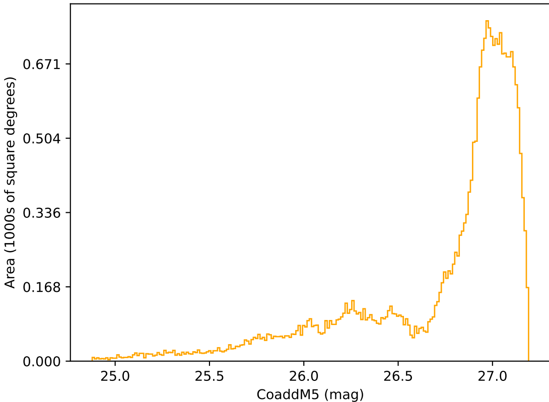
too_elab_r32_d2_griz_v3.4_10yrs All sky r band: CoaddM5
