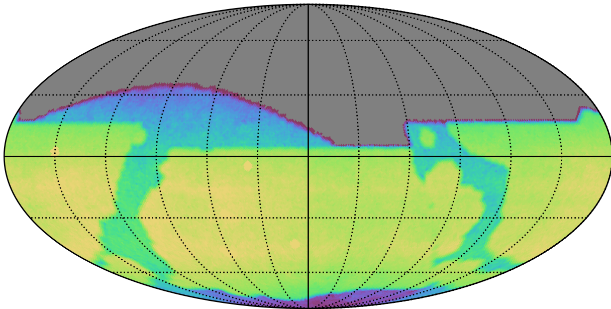
too_elab_r32_d2_griz_v3.4_10yrs All sky i band: CoaddM5
