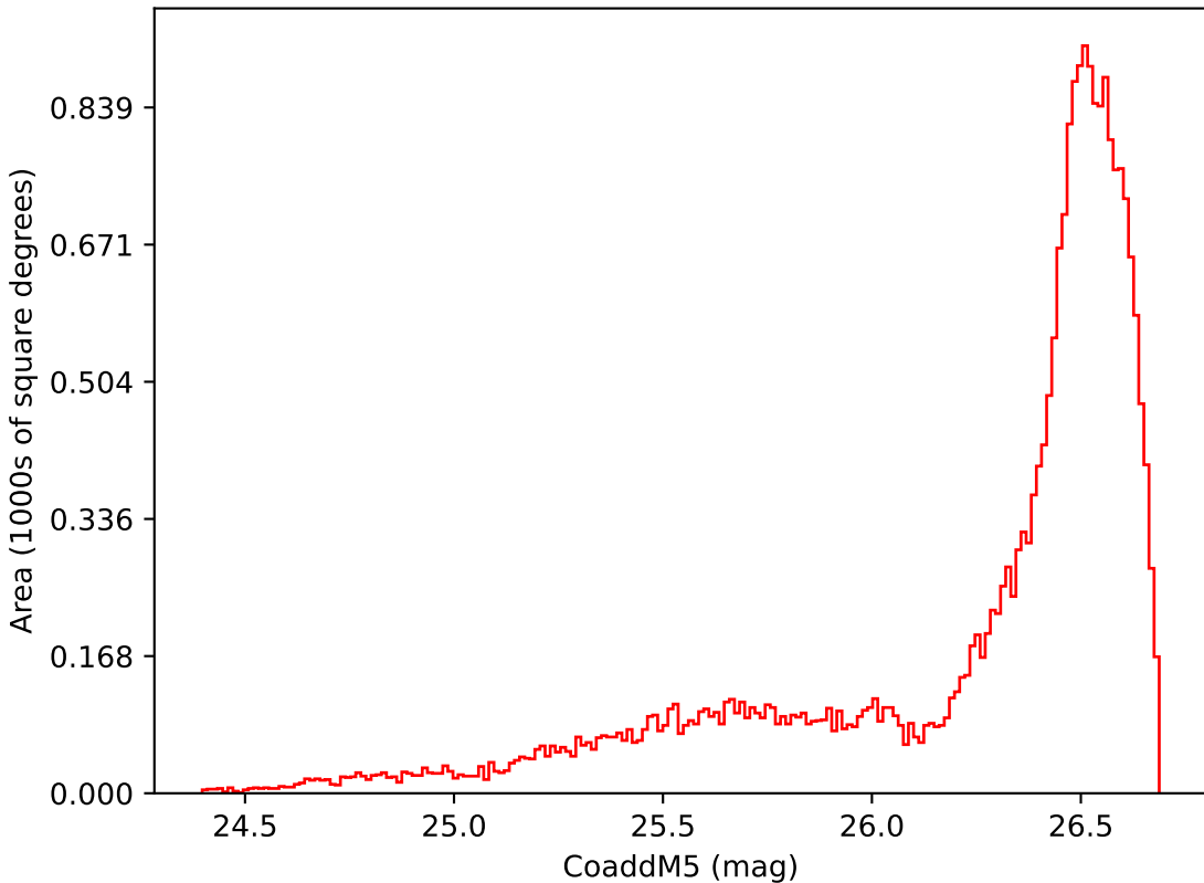
too_elab_r32_d2_griz_v3.4_10yrs All sky i band: CoaddM5
