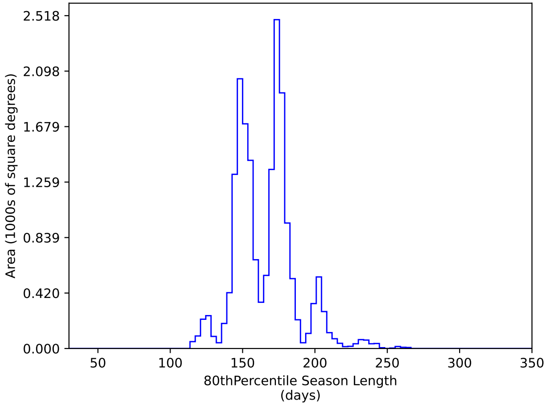
too_elab_r32_d2_griz_v3.4_10yrs WFD y band: 80thPercentile Season Length
