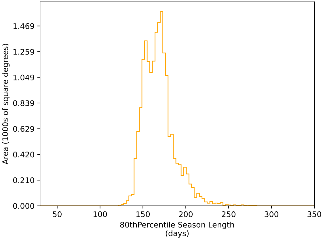
too_elab_r32_d2_griz_v3.4_10yrs WFD r band: 80thPercentile Season Length
