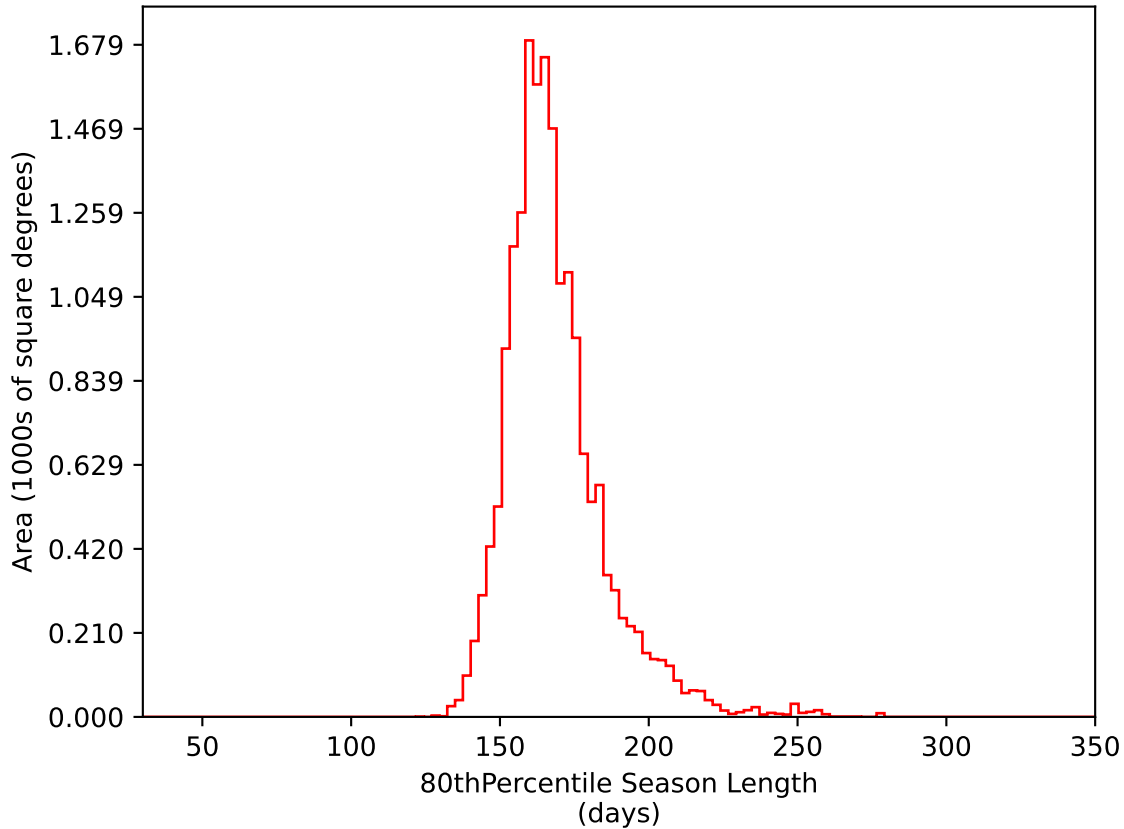
too_elab_r32_d2_griz_v3.4_10yrs WFD i band: 80thPercentile Season Length
