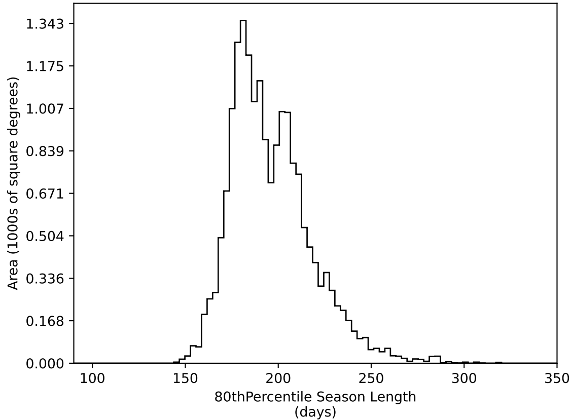
too_elab_r32_d2_griz_v3.4_10yrs WFD all bands: 80thPercentile Season Length
