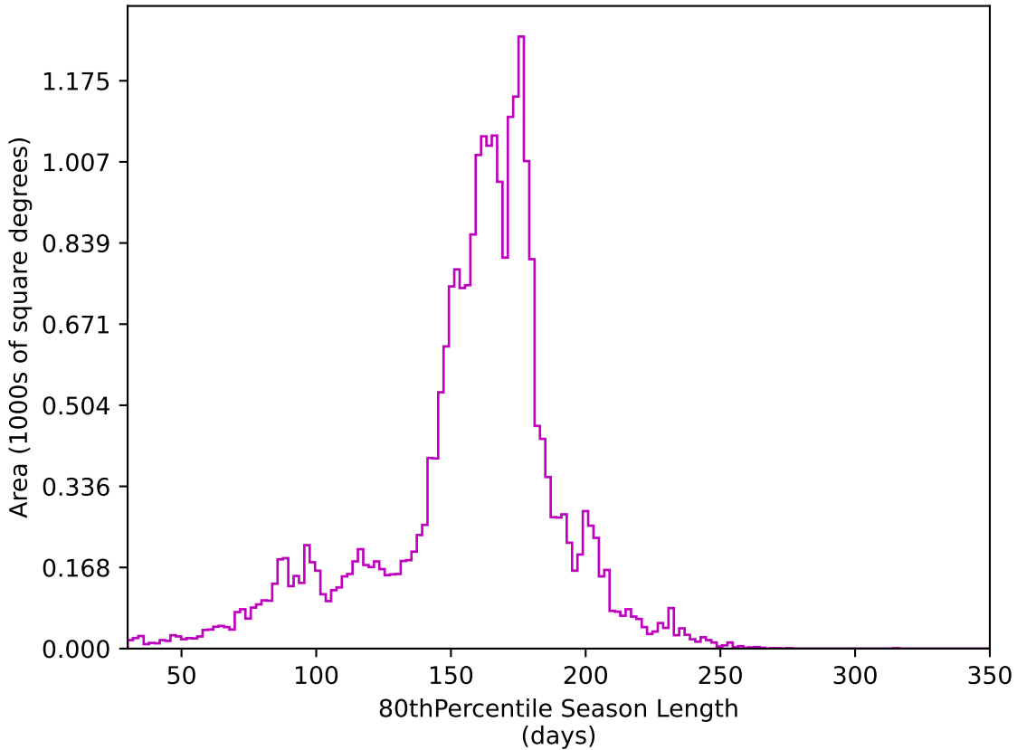
too_elab_r32_d2_griz_v3.4_10yrs All sky z band: 80thPercentile Season Length
