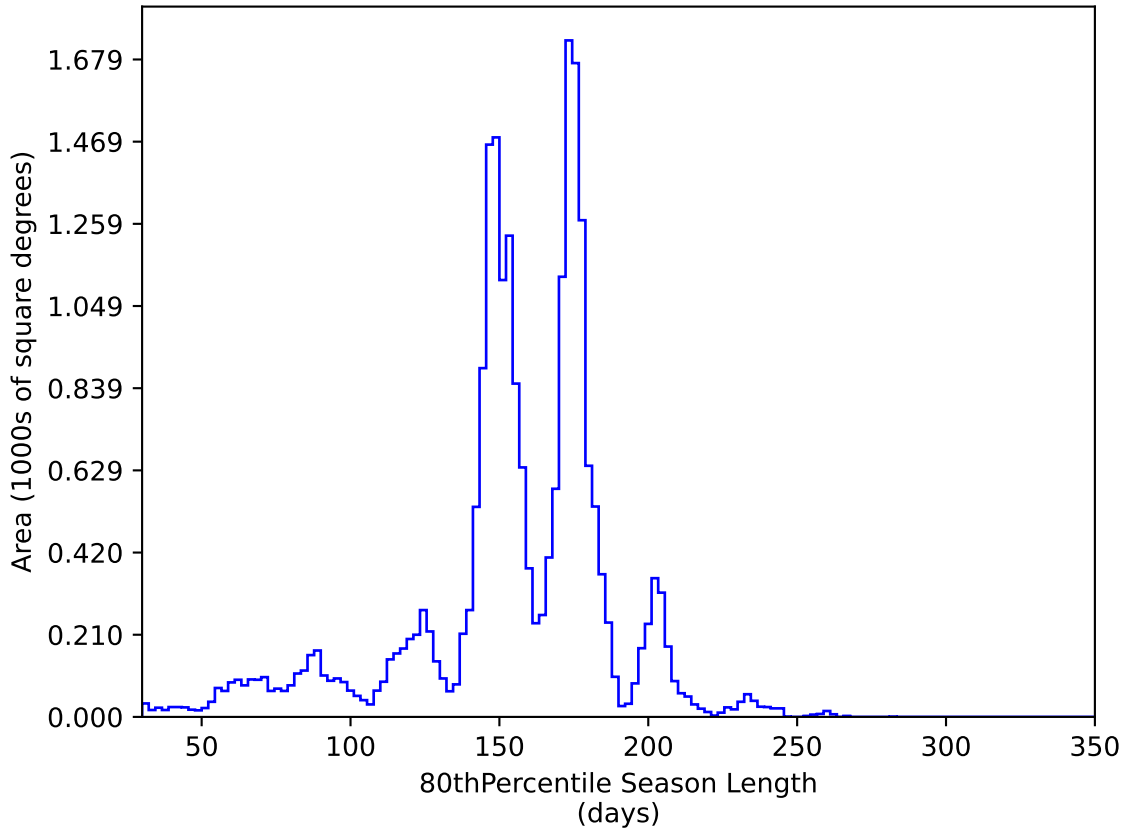
too_elab_r32_d2_griz_v3.4_10yrs All sky y band: 80thPercentile Season Length
