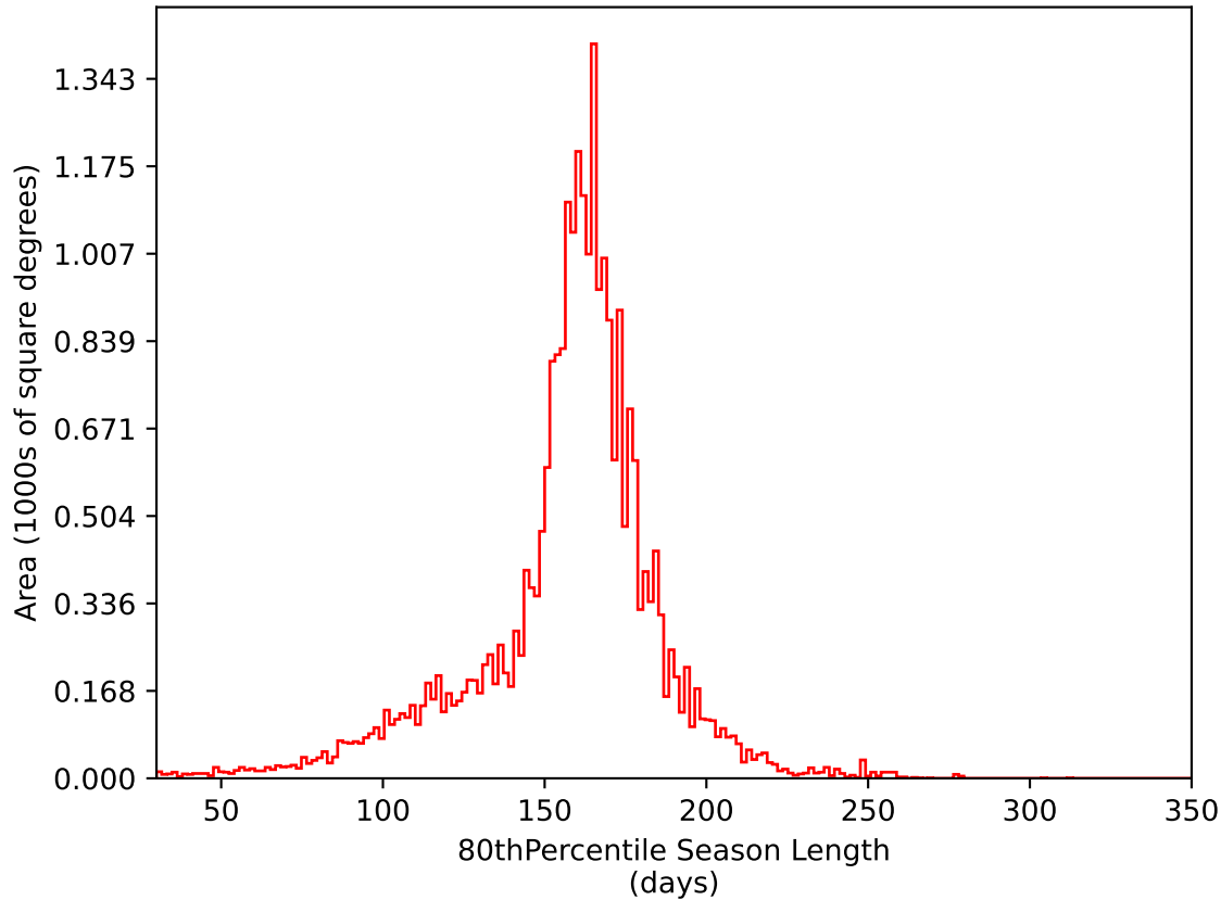
too_elab_r32_d2_griz_v3.4_10yrs All sky i band: 80thPercentile Season Length
