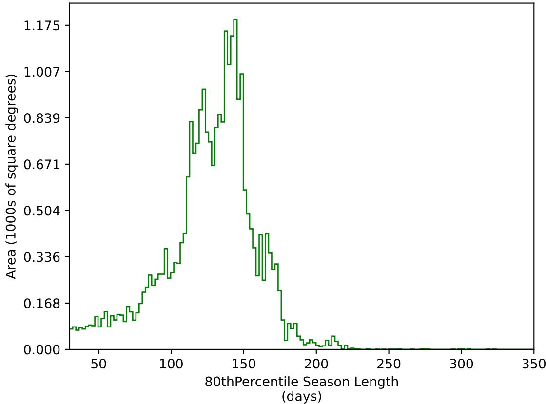
too_elab_r32_d2_griz_v3.4_10yrs All sky g band: 80thPercentile Season Length
