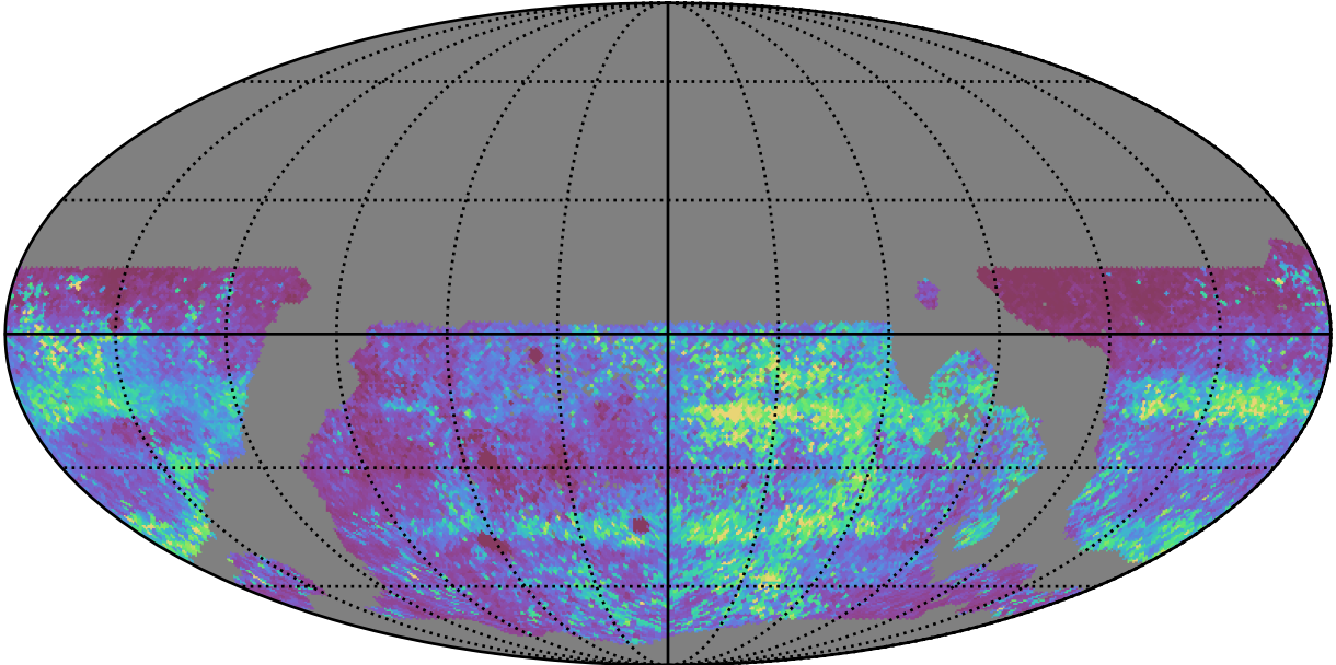
too_elab_r32_d2_griz_v3.4_10yrs WFD zy bands: 75th Percentile Intranight Timespan
