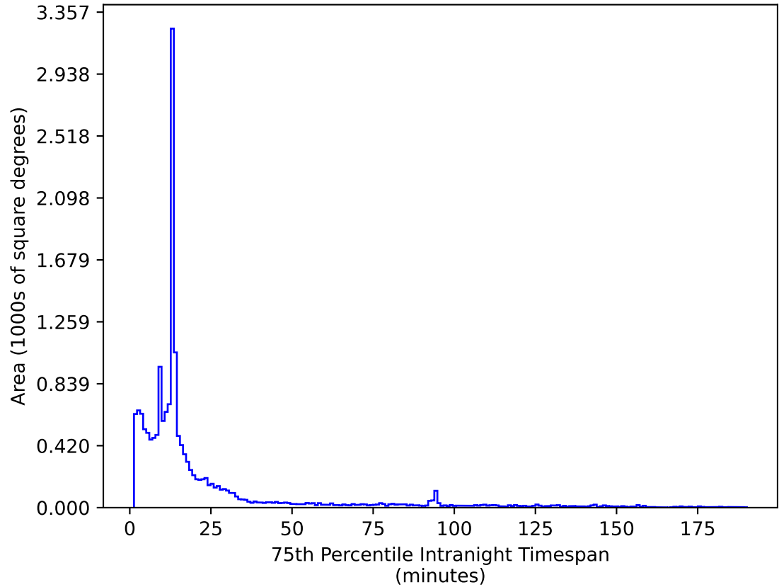
too_elab_r32_d2_griz_v3.4_10yrs WFD z band: 75th Percentile Intranight Timespan
