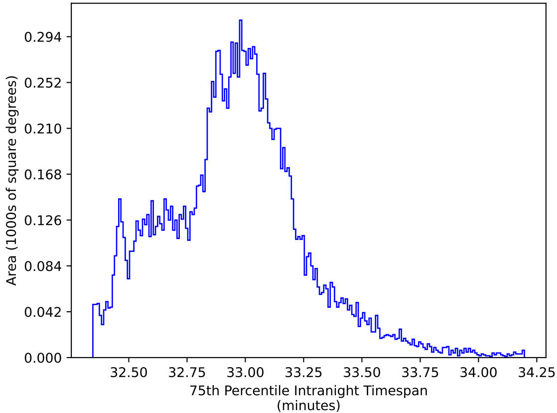
too_elab_r32_d2_griz_v3.4_10yrs WFD y band: 75th Percentile Intranight Timespan
