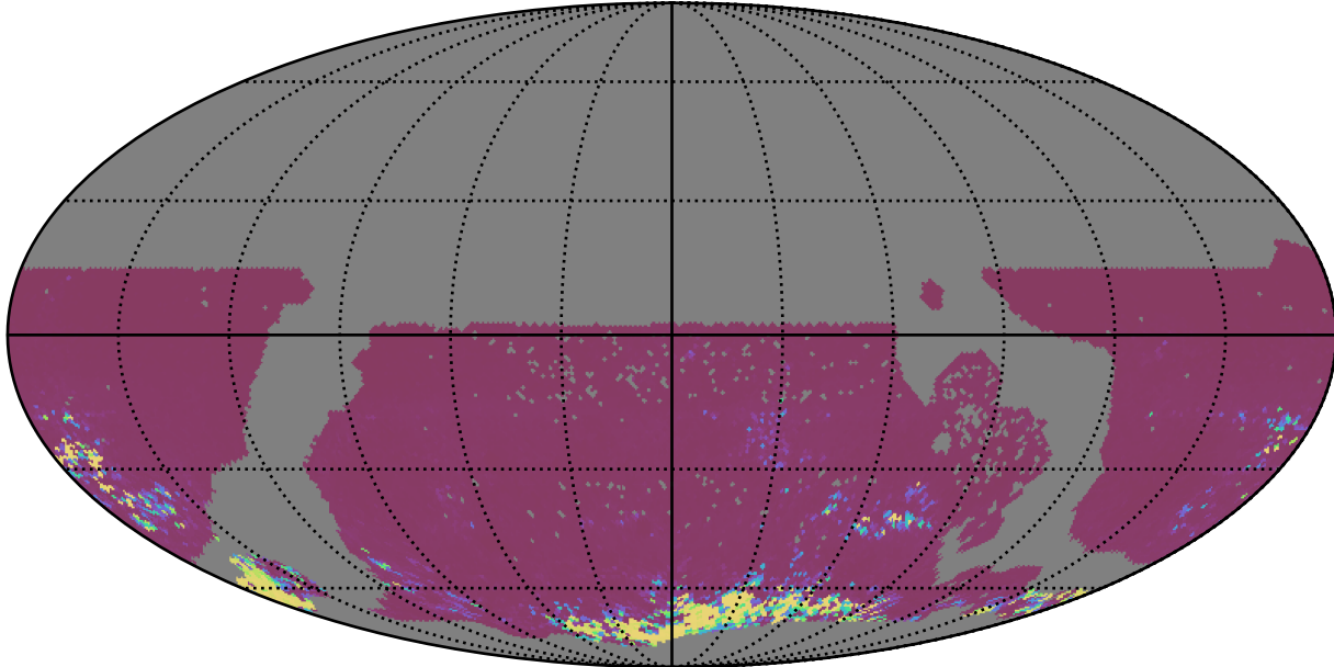
too_elab_r32_d2_griz_v3.4_10yrs WFD ri bands: 75th Percentile Intranight Timespan
