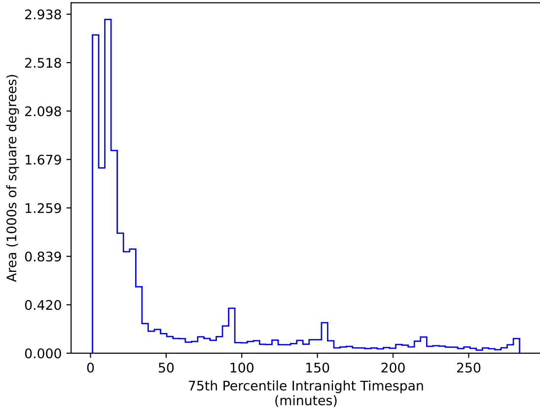
too_elab_r32_d2_griz_v3.4_10yrs WFD r band: 75th Percentile Intranight Timespan
