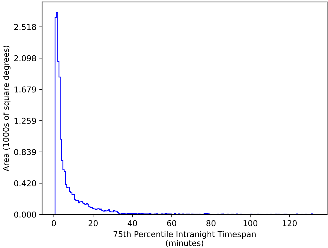
too_elab_r32_d2_griz_v3.4_10yrs WFD g band: 75th Percentile Intranight Timespan
