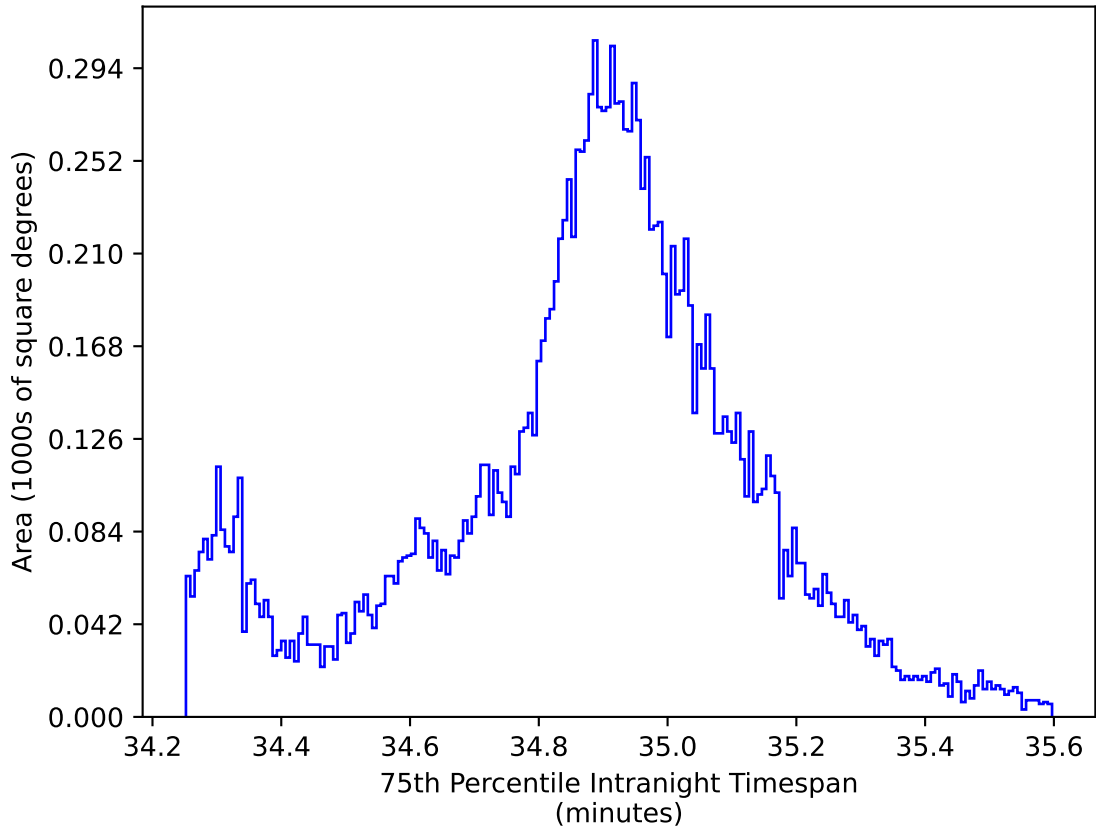
too_elab_r32_d2_griz_v3.4_10yrs WFD all bands: 75th Percentile Intranight Timespan
