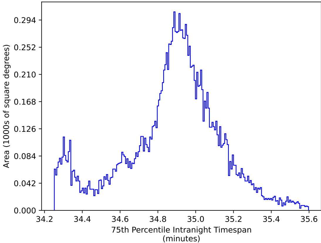
too_elab_r32_d2_griz_v3.4_10yrs WFD: 75th Percentile Intranight Timespan
