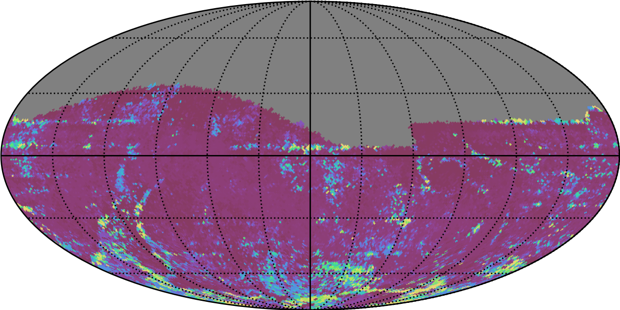
too_elab_r32_d2_griz_v3.4_10yrs All sky z band: 75th Percentile Intranight Timespan
