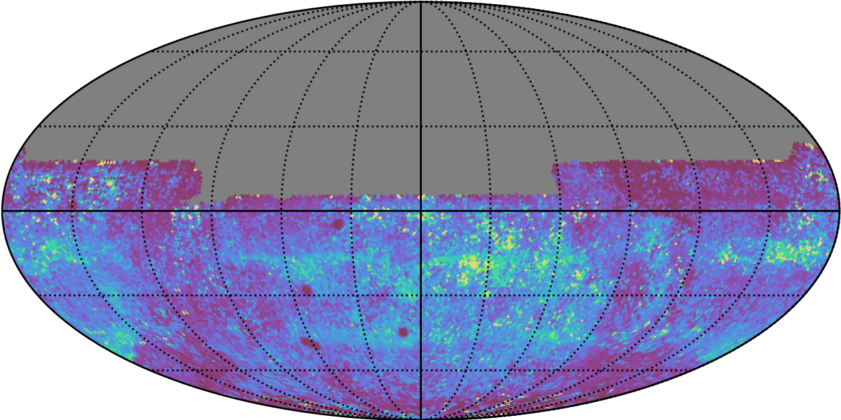
too_elab_r32_d2_griz_v3.4_10yrs All sky y band: 75th Percentile Intranight Timespan
