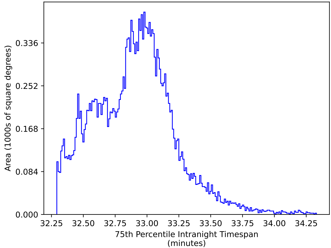
too_elab_r32_d2_griz_v3.4_10yrs All sky y band: 75th Percentile Intranight Timespan
