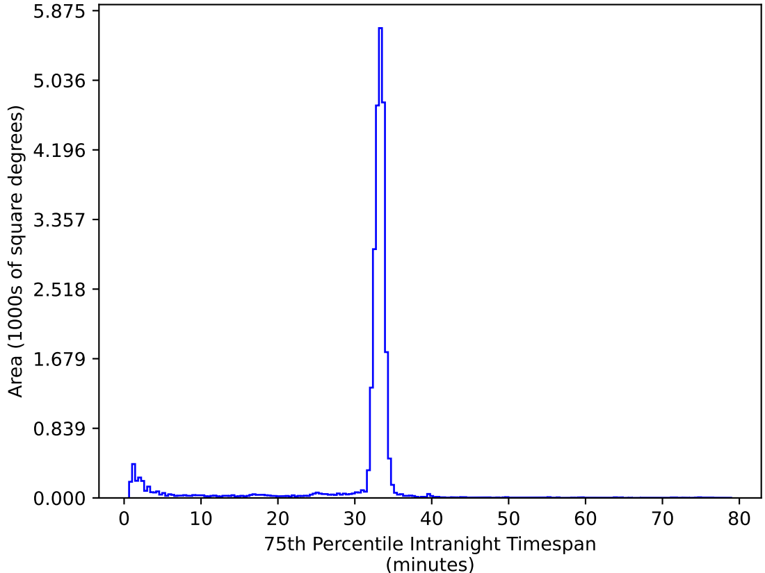
too_elab_r32_d2_griz_v3.4_10yrs All sky ug bands: 75th Percentile Intranight Timespan
