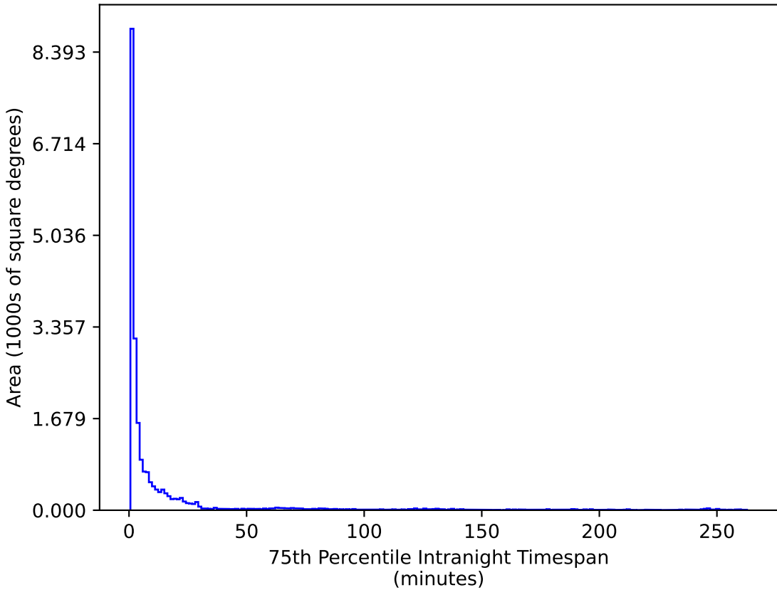
too_elab_r32_d2_griz_v3.4_10yrs All sky u band: 75th Percentile Intranight Timespan
