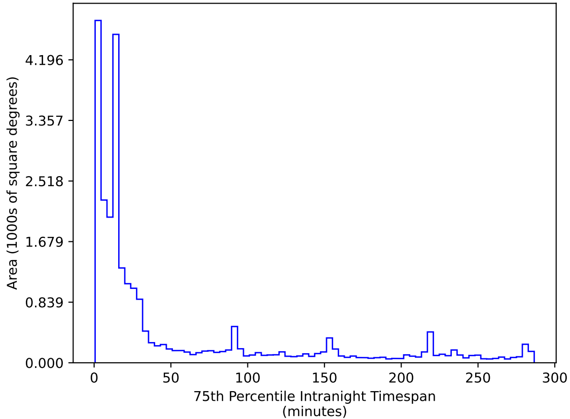
too_elab_r32_d2_griz_v3.4_10yrs All sky r band: 75th Percentile Intranight Timespan
