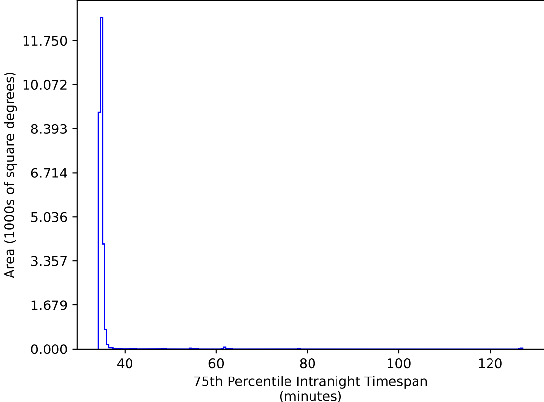
too_elab_r32_d2_griz_v3.4_10yrs All sky iz bands: 75th Percentile Intranight Timespan
