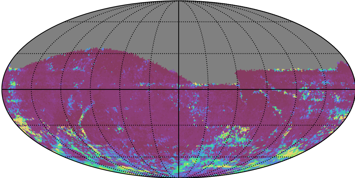
too_elab_r32_d2_griz_v3.4_10yrs All sky i band: 75th Percentile Intranight Timespan
