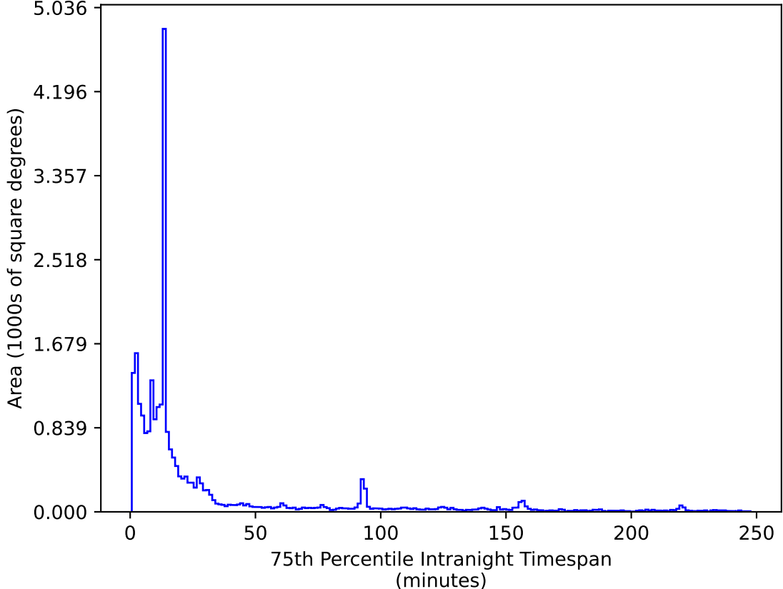
too_elab_r32_d2_griz_v3.4_10yrs All sky i band: 75th Percentile Intranight Timespan
