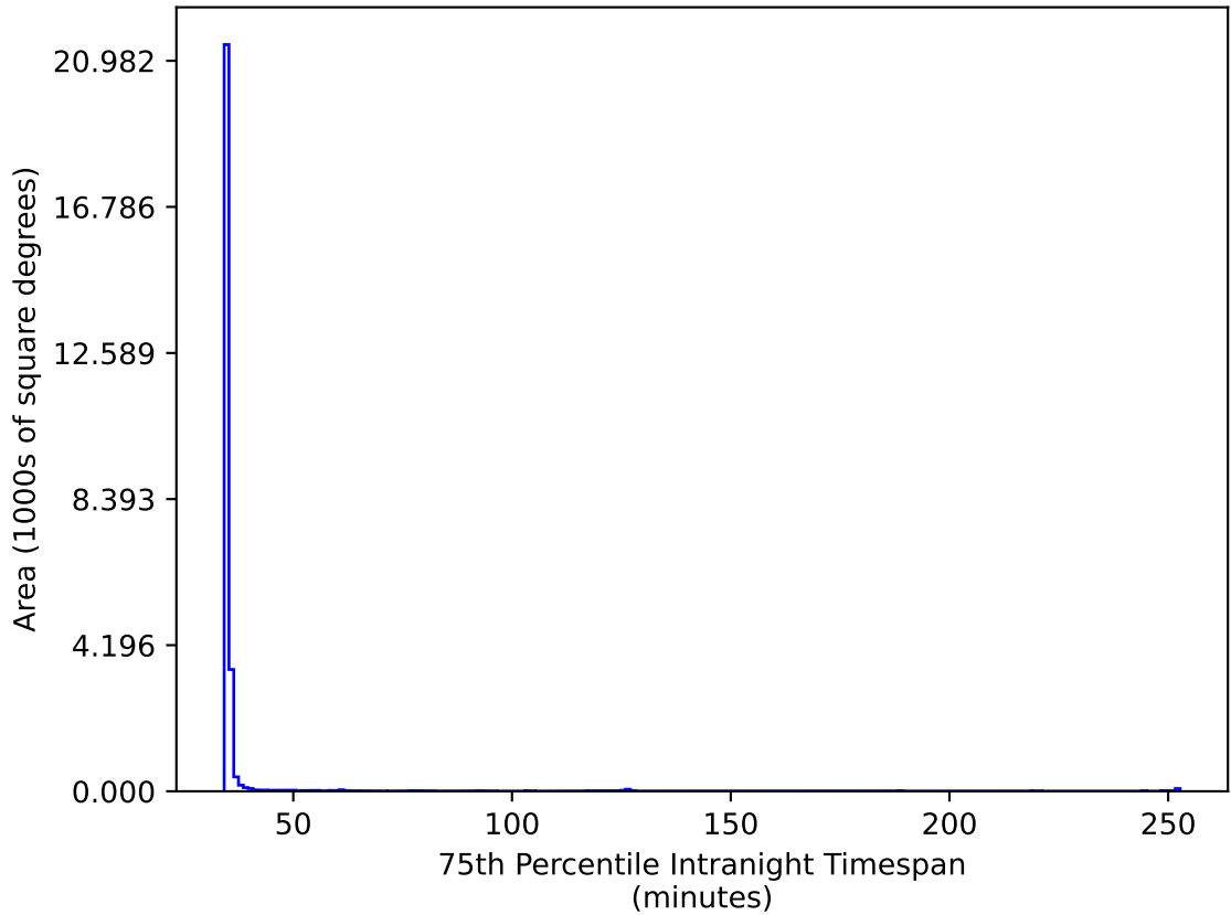
too_elab_r32_d2_griz_v3.4_10yrs All sky gr bands: 75th Percentile Intranight Timespan
