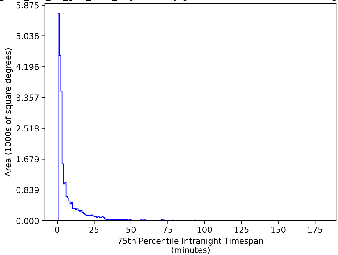
too_elab_r32_d2_griz_v3.4_10yrs All sky g band: 75th Percentile Intranight Timespan
