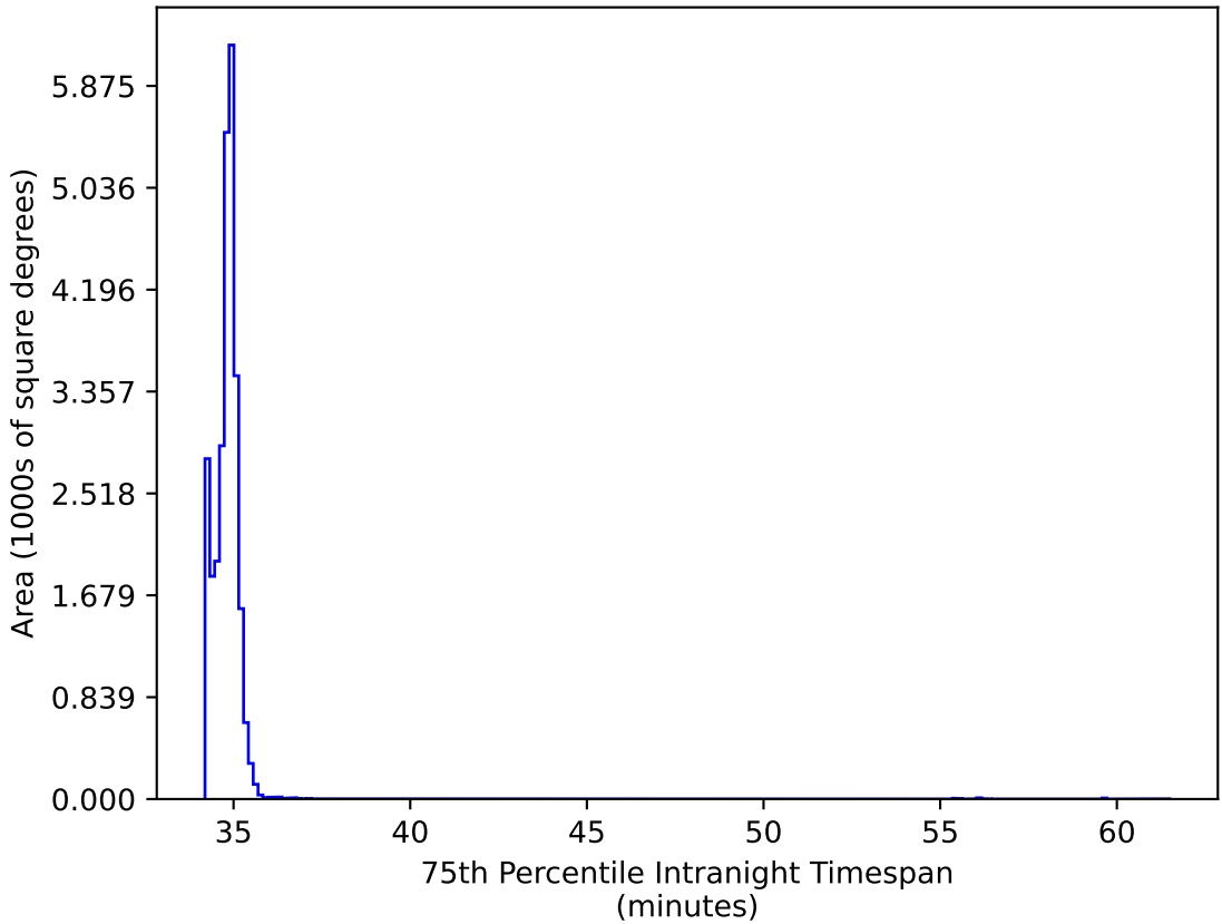
too_elab_r32_d2_griz_v3.4_10yrs All sky all bands: 75th Percentile Intranight Timespan
