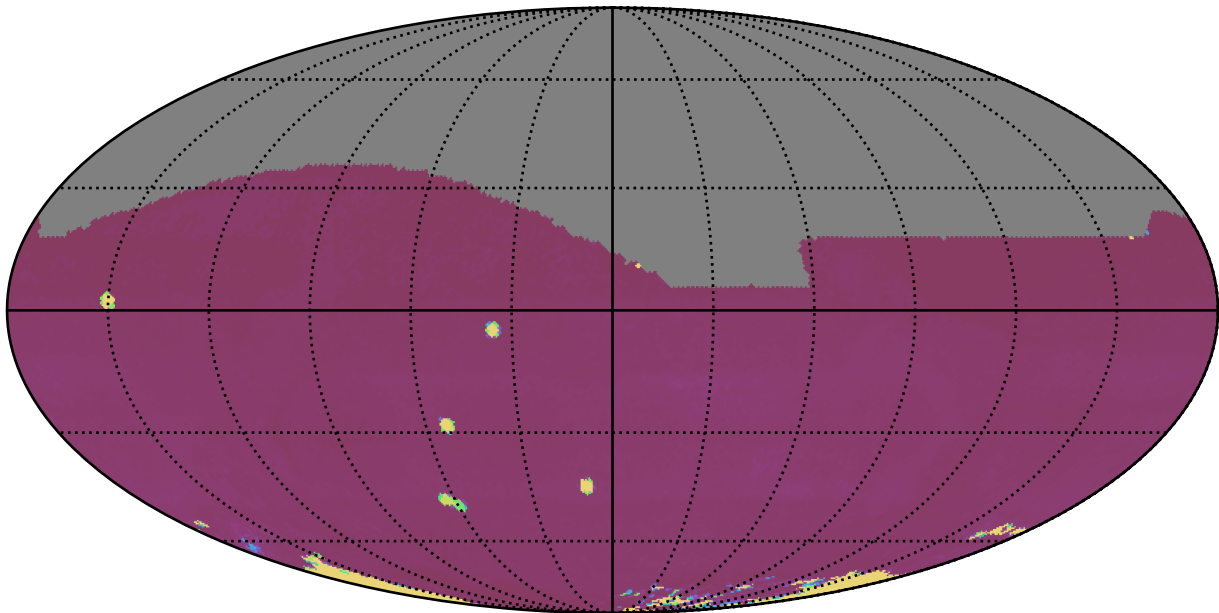
too_elab_r32_d2_griz_v3.4_10yrs All sky: 75th Percentile Intranight Timespan
