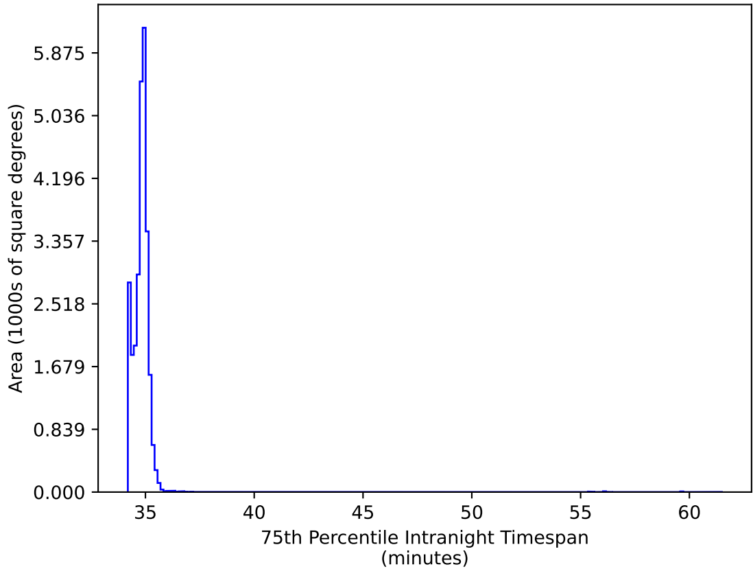
too_elab_r32_d2_griz_v3.4_10yrs All sky: 75th Percentile Intranight Timespan
