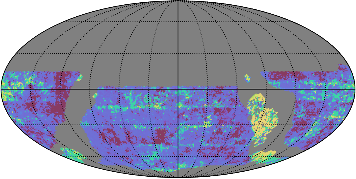
too_elab_r32_d2_griz_v3.4_10yrs WFD y band: 20thPercentile Inter-Night Gap
