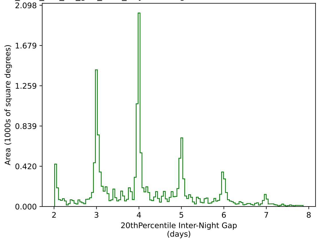
too_elab_r32_d2_griz_v3.4_10yrs WFD g band: 20thPercentile Inter-Night Gap
