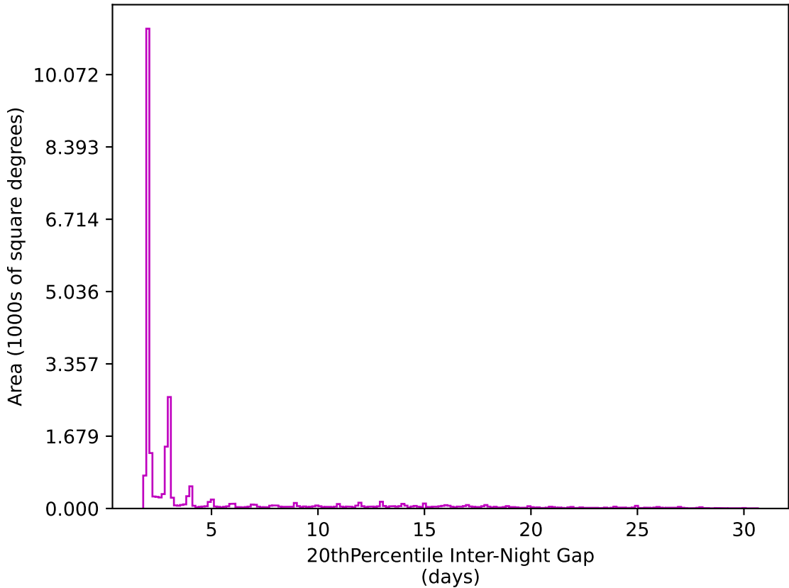
too_elab_r32_d2_griz_v3.4_10yrs All sky z band: 20thPercentile Inter-Night Gap
