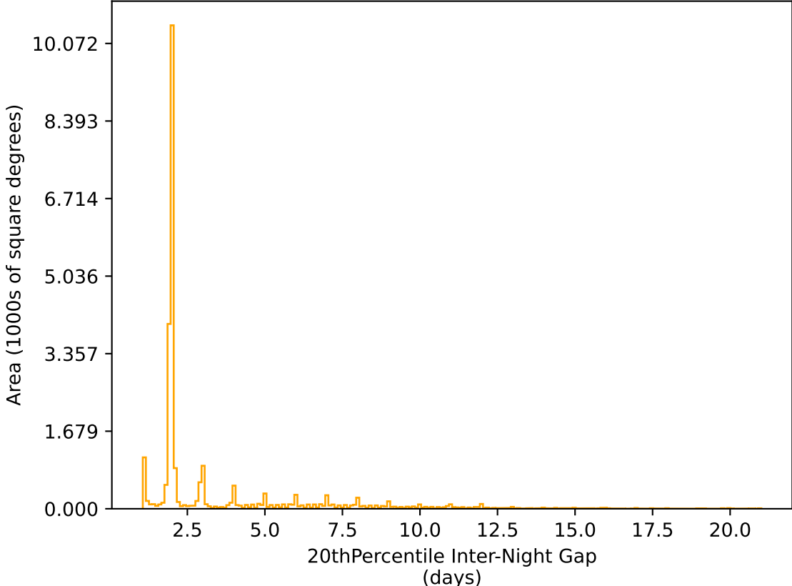
too_elab_r32_d2_griz_v3.4_10yrs All sky r band: 20thPercentile Inter-Night Gap
