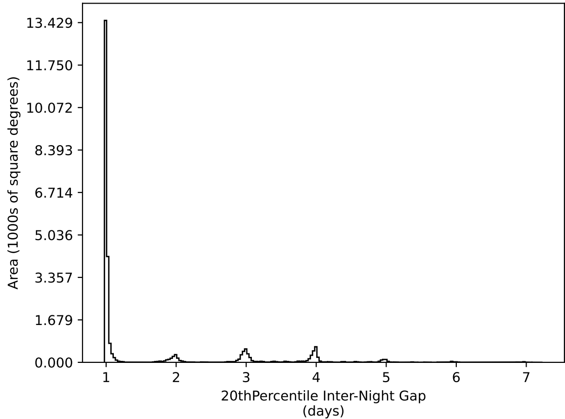
too_elab_r32_d2_griz_v3.4_10yrs All sky all bands: 20thPercentile Inter-Night Gap
