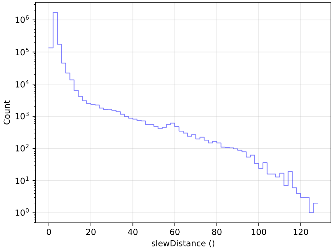
too_elab_r32_d2_griz_v3.4_10yrs All visits: Slew Distance Histogram
