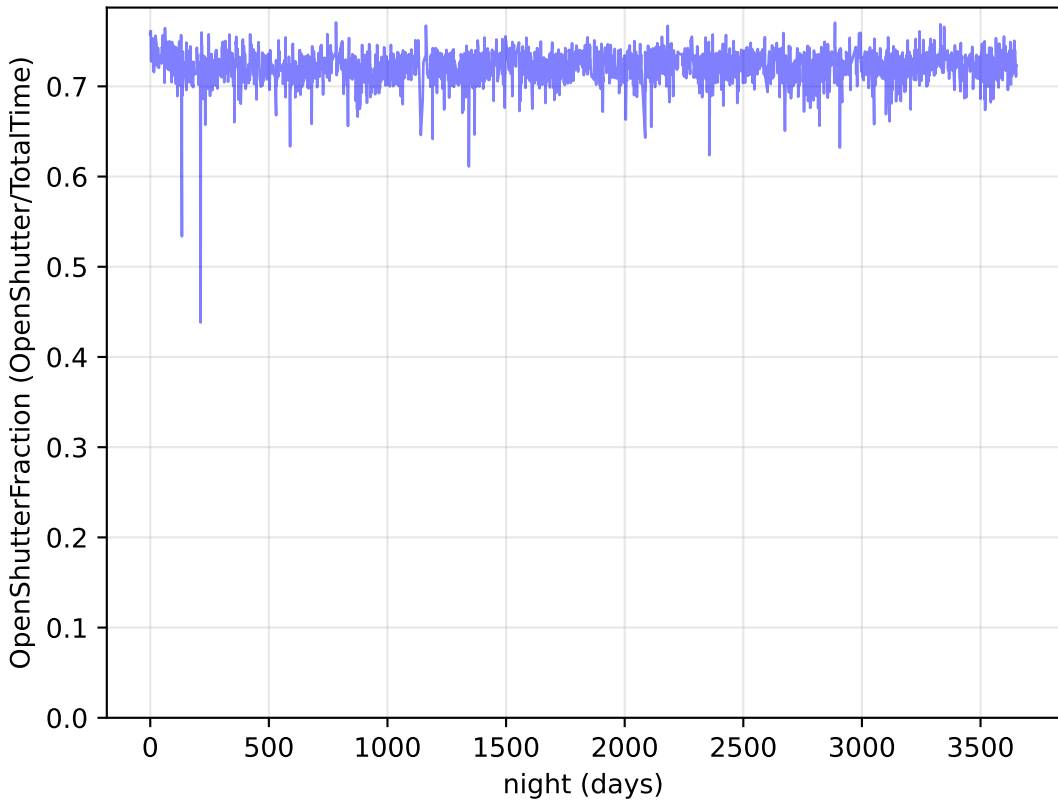
too_elab_r32_d2_griz_v3.4_10yrs : OpenShutterFraction
