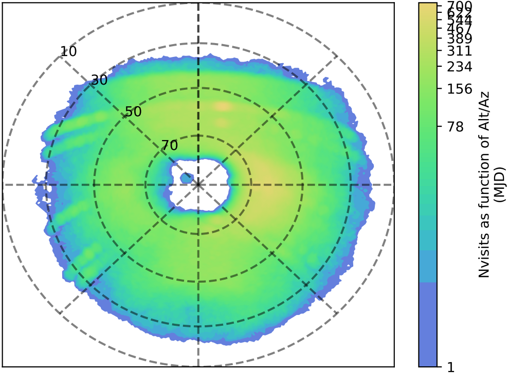
too_elab_r32_d2_griz_v3.4_10yrs u: Nvisits as function of Alt/Az
