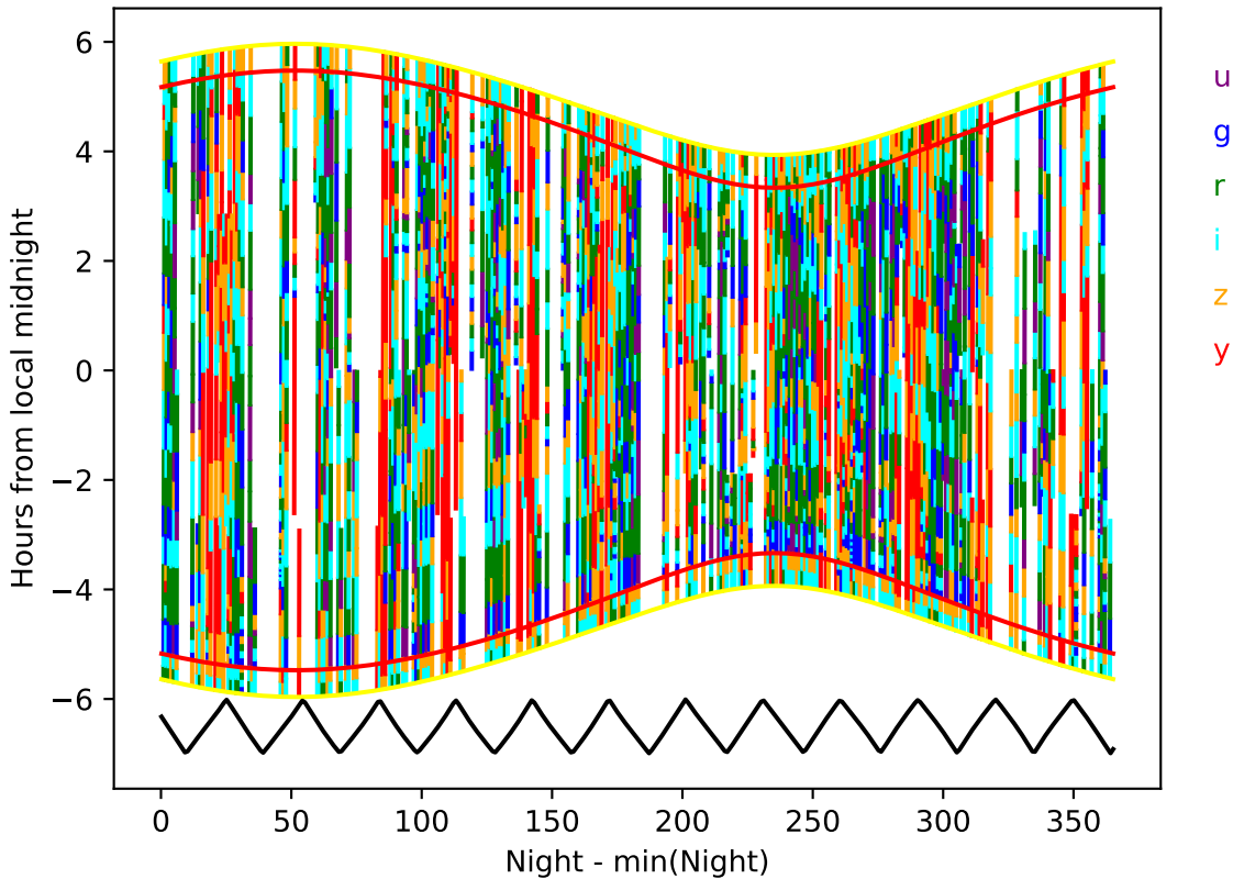
too_elab_r32_d2_griz_v3.4_10yrs year 7-8: Hourglass
