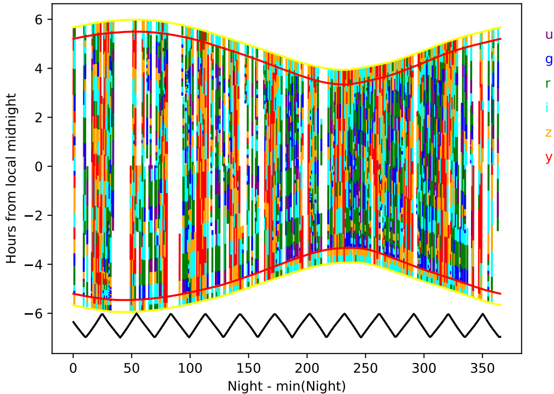
too_elab_r32_d2_griz_v3.4_10yrs year 4-5: Hourglass
