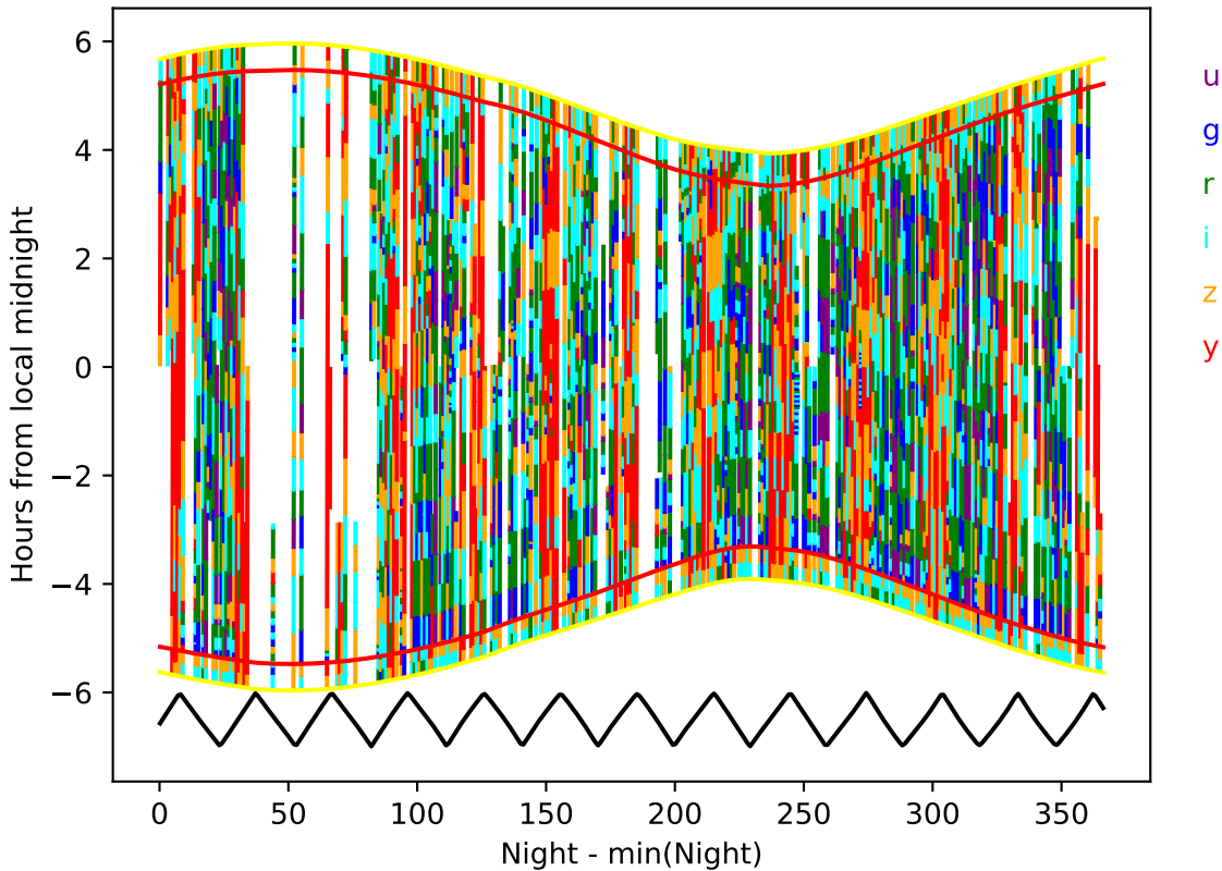
too_elab_r32_d2_griz_v3.4_10yrs year 3-4: Hourglass
