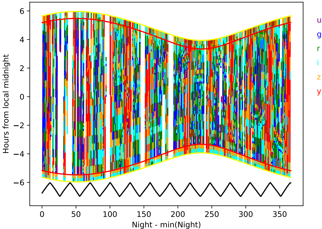
too_elab_r32_d2_griz_v3.4_10yrs year 0-1: Hourglass
