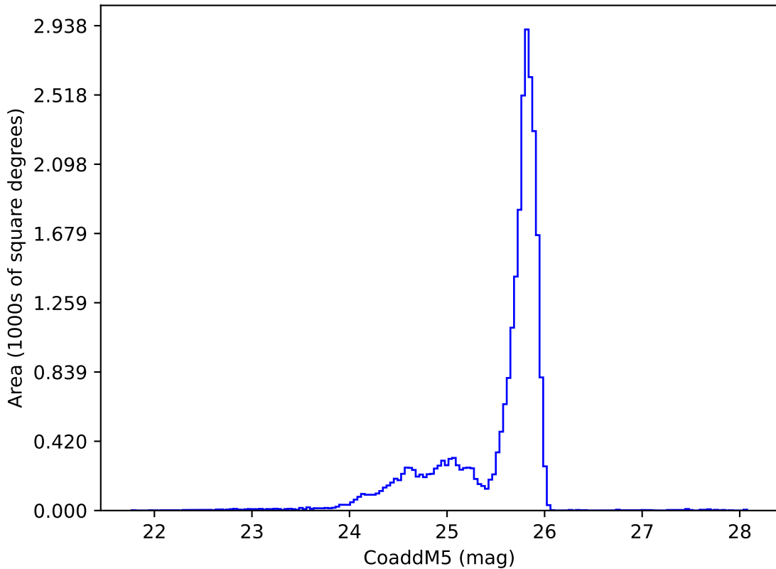
too_elab_r32_d2_griz_v3.4_10yrs z: CoaddM5
