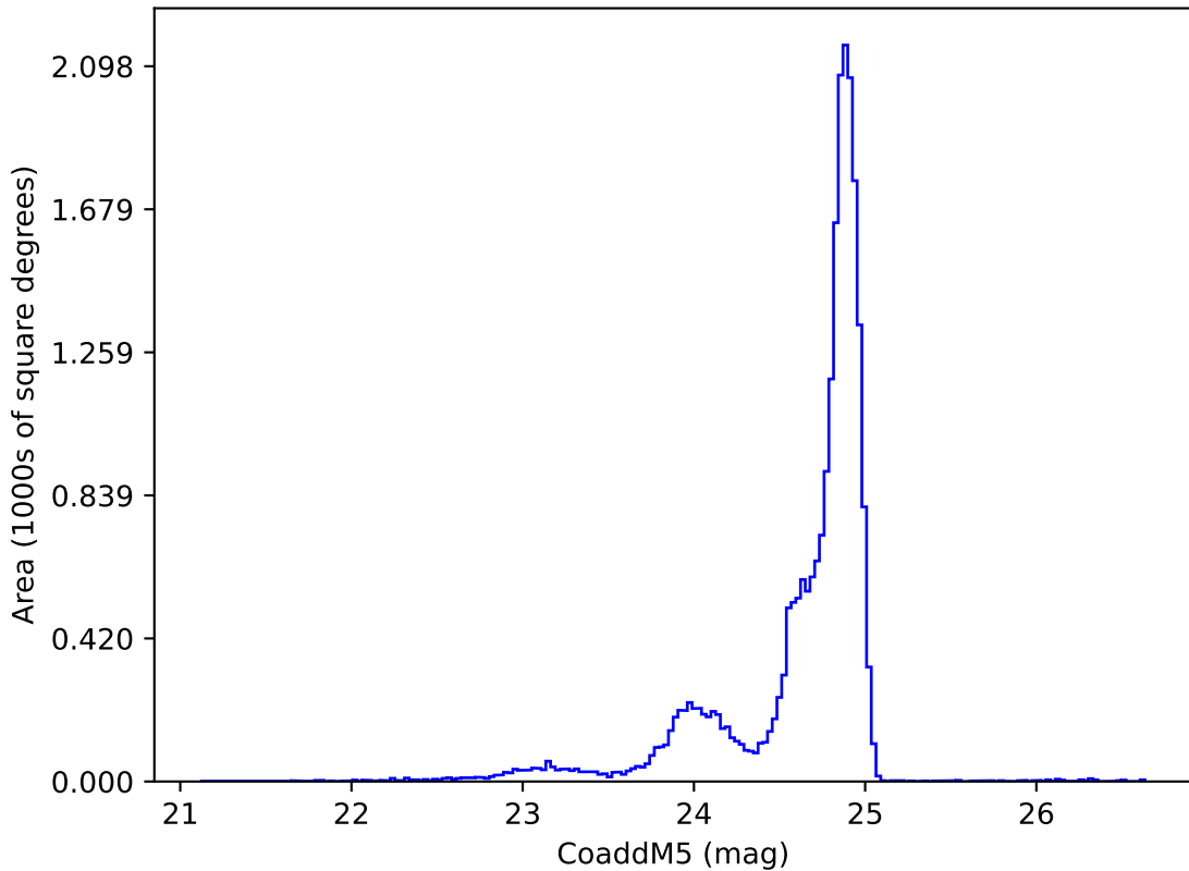
too_elab_r32_d2_griz_v3.4_10yrs y: CoaddM5
