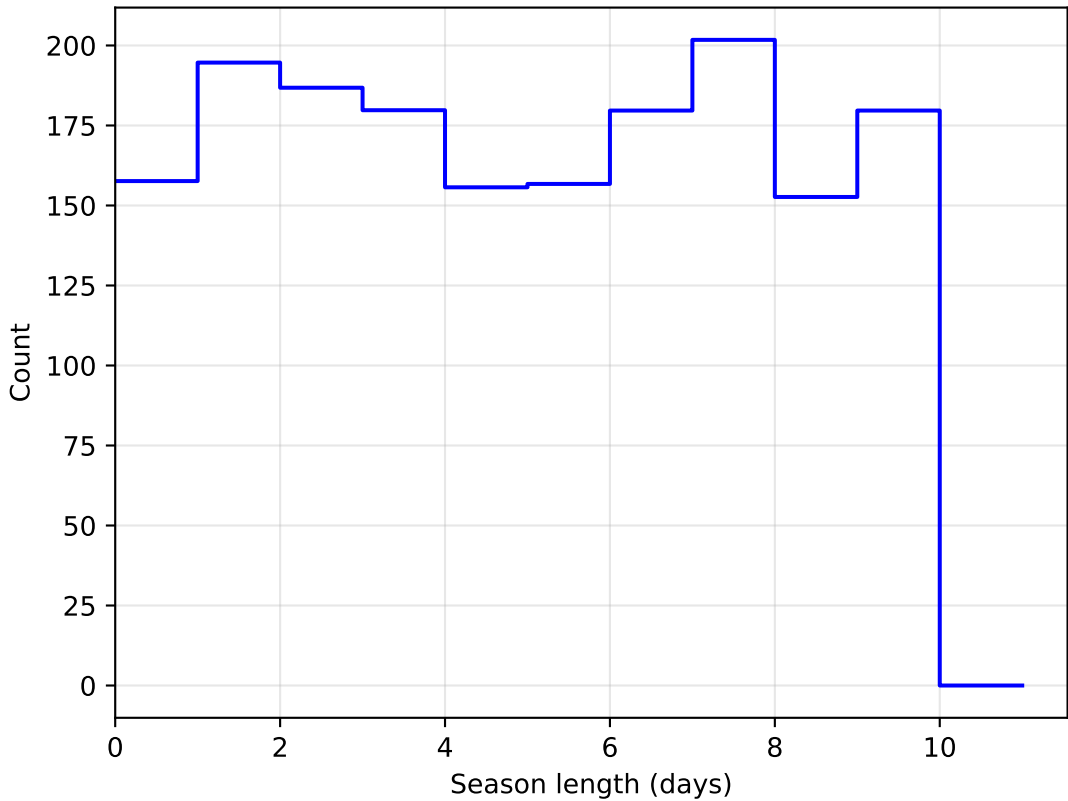
too_elab_r32_d2_griz_v3.4_10yrs DD:WFD all bands: SeasonLength
